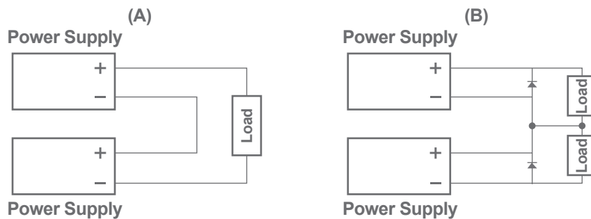
3.3.1 The example of series operation & parallel operation
