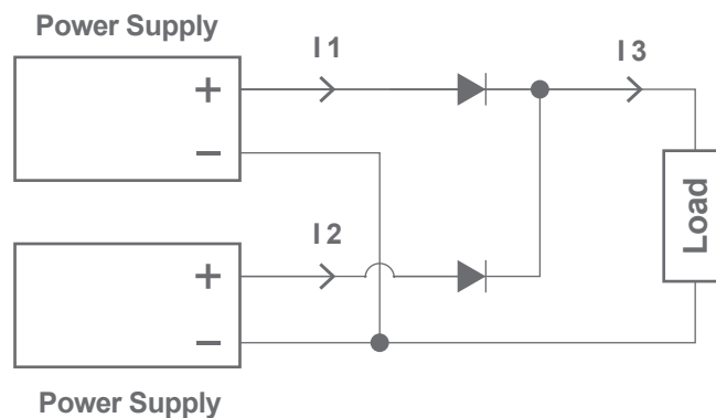
3.3.2 The example of parallel operation/loge-term operation
