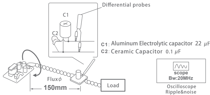
1.5.1 UUHP150 | Example of measuring output ripple & noise
