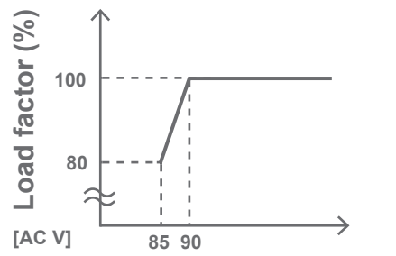
2.5.3 Input derating curve
