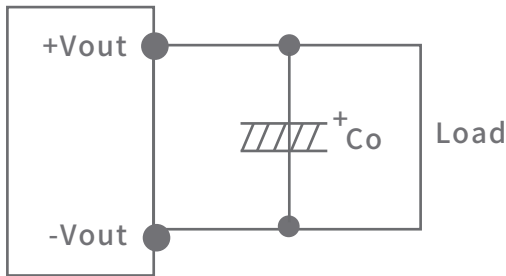
3.4.1 The example of connect an external capacitor to the output
