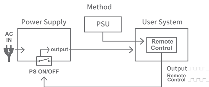
3.2.1 The example of remote ON/OFF
