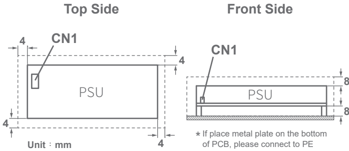
2.1.1 UUHP | The installation distance of open frame
