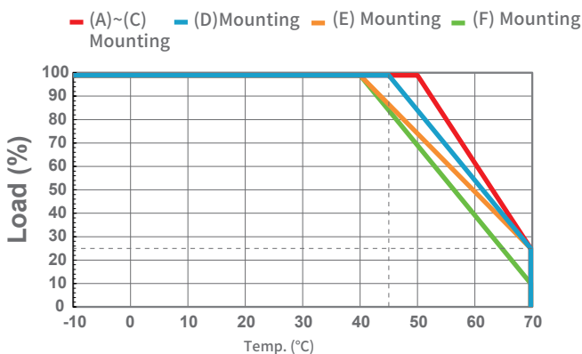
2.5.2 Mounting direction output derating curve
